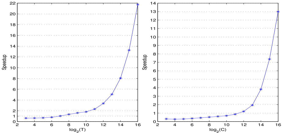
Figure 4: On the left: speedup obtained using zero-delay convolution for the stochastic shortest path problem as formulated in (2) and (3), for a random network with n = 10 nodes and m = 40 edges, with the length distribution L_{ij} of each edge (i, j) chosen by sampling a random vector in [0, 1]^T and normalizing it. On the right: speedup obtained using zero-delay convolution for the stochastic knapsack problem as formulated in (6) and (7), for a random instance with n = 10 items, each with a random value in [0, 1] and a size distribution sampled from [0, 1]^C and normalized. As expected from the theoretical analysis of these algorithms, the speedup obtained using zero-delay convolution is largely independent of n and m (on the left) and of n (on the right). We observed very slight increases in speedup for larger values of n and m , attributable to caching artifacts.
