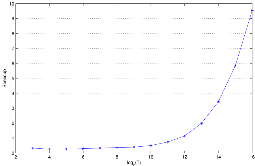
Figure 2: Speedup obtained by using zero-delay convolution for different values of T (we use powers of two, since these are best suited for the FFT; performance is slightly worse for FFT-based approaches if using a problem size that is not a power of two, especially a problem size just larger than a power of two).
