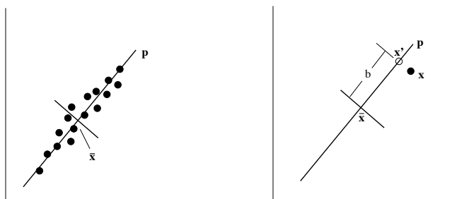
Figure 16: Applying a PCA to a set of 2D vectors. \mathbf{p} is the principal axis. Any point \mathbf{x} can be approximated by the nearest point on the line, \mathbf{x}' (see text).
