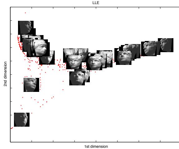
Figure 1.4: LLE applied ( k = 5 ) to the same data set. A two-dimensional projection is shown, with a sample of the original input images.
