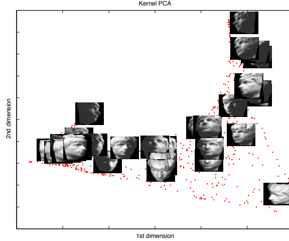
Figure 1.3: Kernel PCA with Gaussian kernel applied to the same data set. A two-dimensional projection is shown, with a sample of the original input images.
