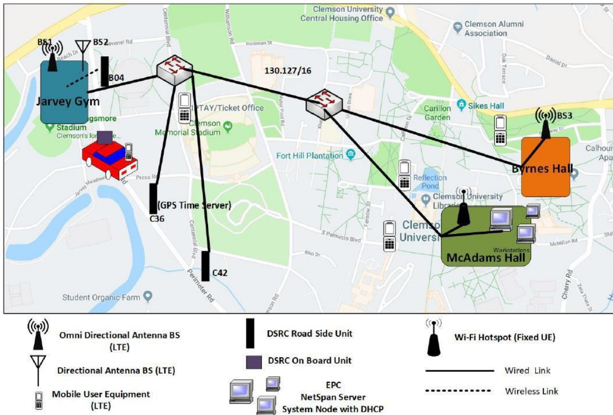
Fig. 9. Radio Access Network of Clemson University LTE Network.
