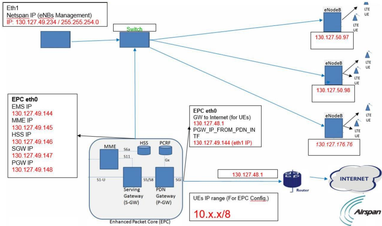
Fig. 6. Clemson University LTE Network Architecture.
