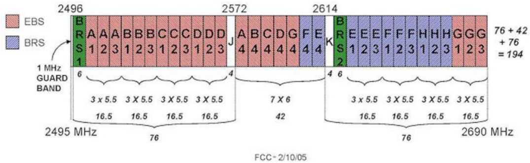
Fig. 7. BRS-EBS Band Plans (Post-Transition at 2496-2690 MHz).
