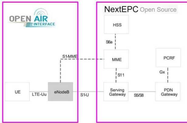
Fig. 12. Simulated end-to-end LTE network.
