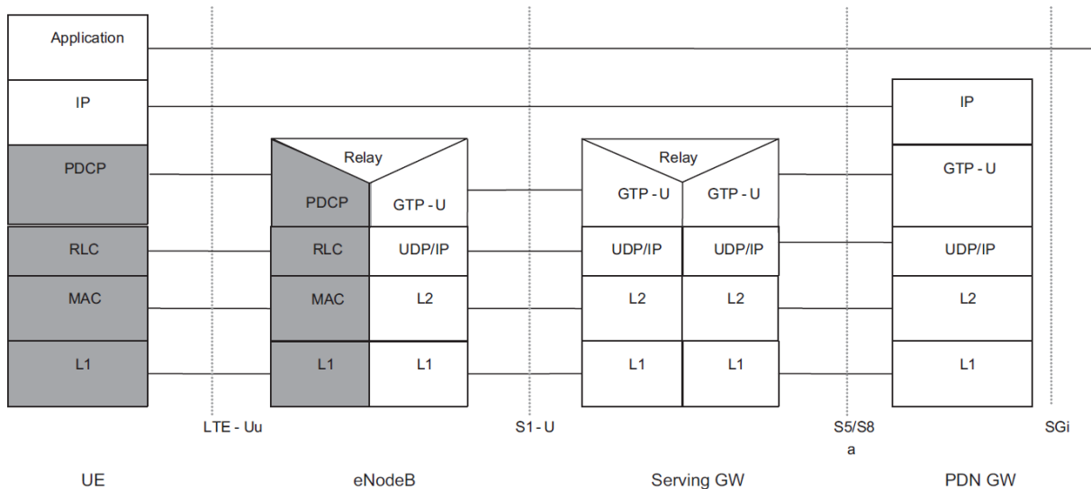
Fig. 4. The E-UTRAN user plane protocol stack.
