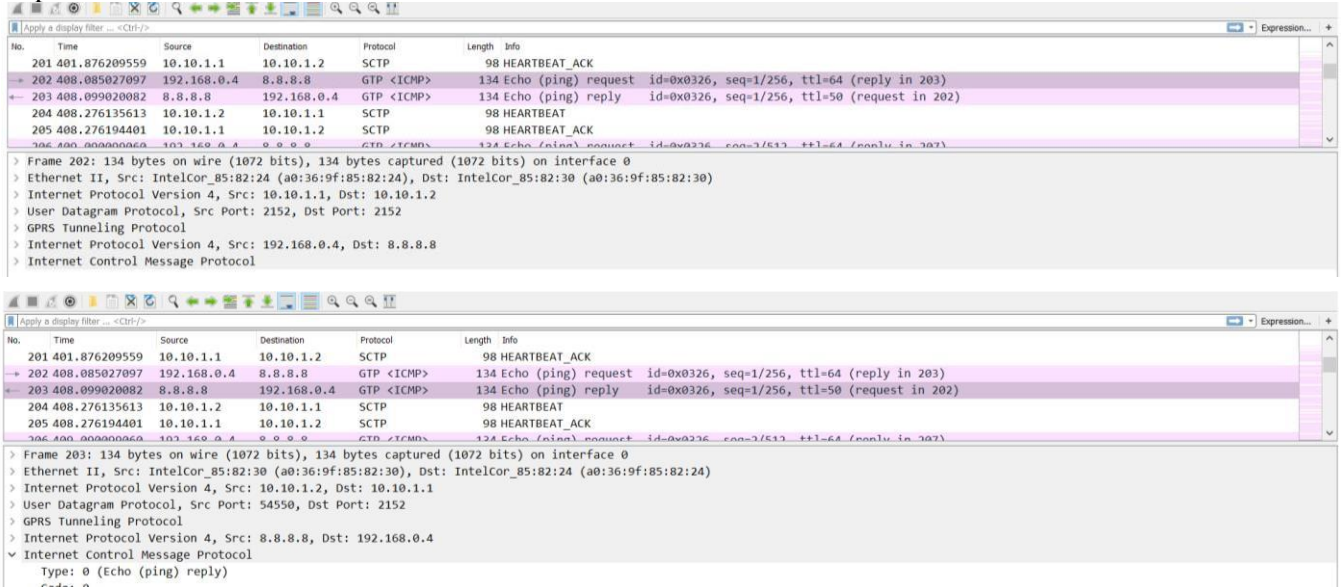
Fig. 19. Wireshark trace for A) Ping request. B) Ping reply.
