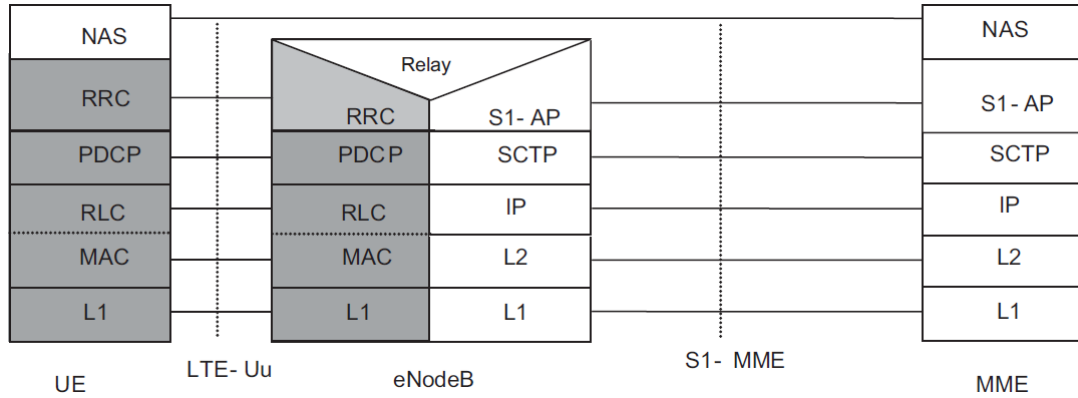
Fig. 5. Control plane protocol stack.
