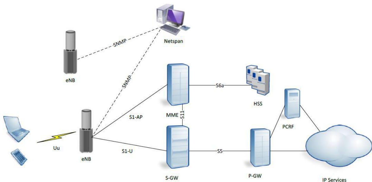
Fig. 10. Netspan Management of LTE eNodeBs.
