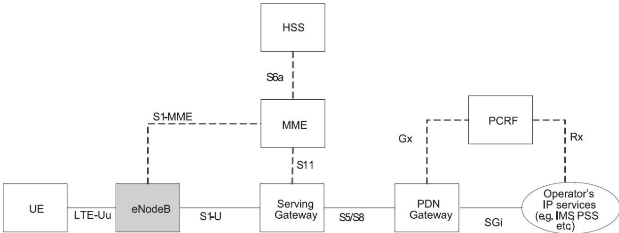
Fig. 2. The EPS network elements.
