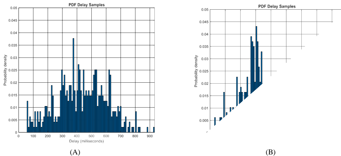
Fig. 23. Comparison of RTT: A) Commercial LTE vs B) WiFi
