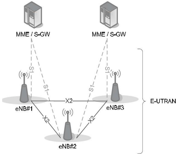
Fig. 3. Overall E-UTRAN architecture.
