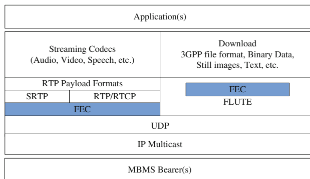
Fig. 1 3GPP MBMS protocol stack
