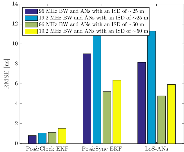
Fig. 9. Average RMSEs for the UN clock offset estimates along 15 different random routes through the Madrid map, with synchronous (left) and unsynchronous (middle) ANs. Also shown are the respective RMSEs for the LoS-ANs mutual clock offset estimates (right).
