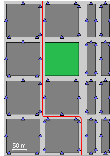
Fig. 4. Madrid map with example AN deployment (blue triangles) and UN trajectory (red path).
