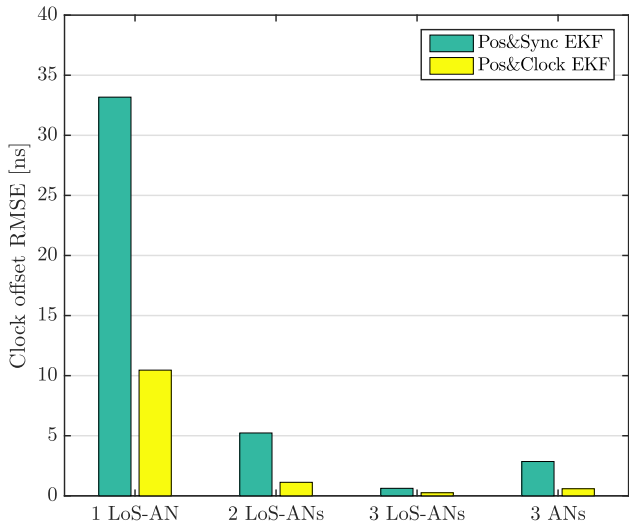
Fig. 11. Average RMSEs for the UN clock offset estimates along 15 different random routes through the Madrid map, with different number of LoS-ANs and under imperfect LoS-detection (denoted as 3 ANs).
