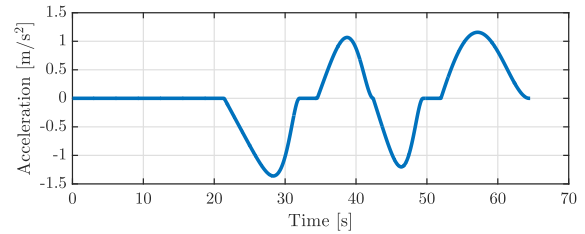
Fig. 6. Acceleration profile for the example UN trajectory shown in Fig. 4.
