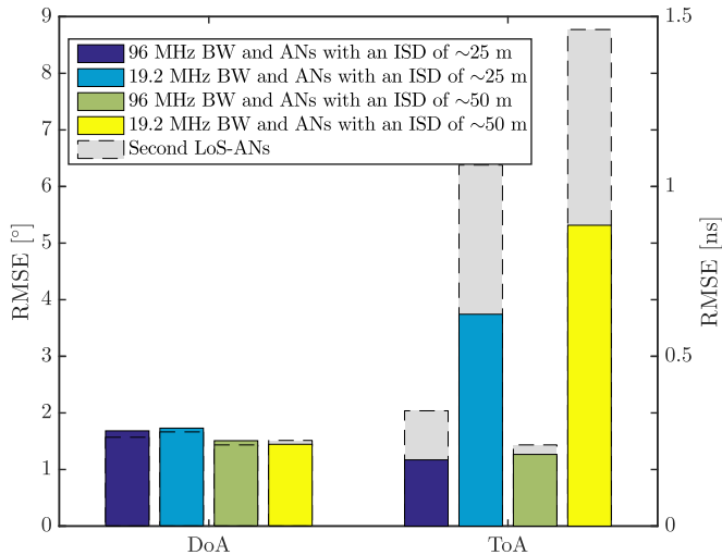
Fig. 7. Average RMSEs for the estimated azimuth DoA and ToA at the closest LoS-ANs (colored bars) and the second LoS-ANs (gray bars) along 15 different random routes through the Madrid map.
