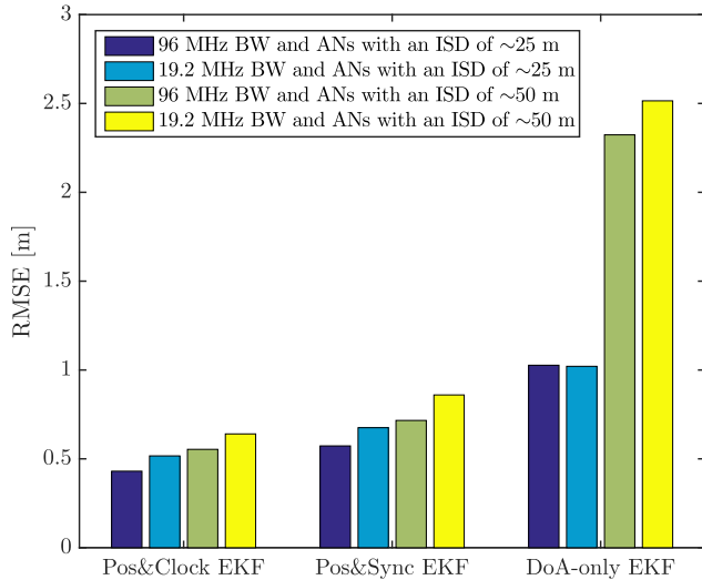
Fig. 8. Positioning RMSEs for all tracking methods and with different simulation numerologies, along 15 different random routes taken through the Madrid map.
