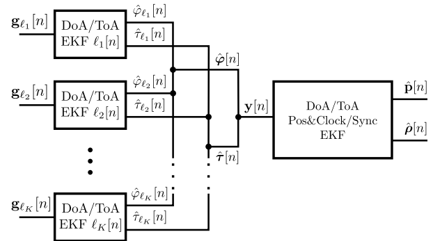
Fig. 2. Cascaded EKFs for joint UN positioning and network clock synchronization. The DoA/ToA EKFs operate in a distributed manner at each AN while the Pos&Clock/Sync EKFs operate in a central-unit fusing the azimuth DoA and ToA measurements of K[n] ANs.
