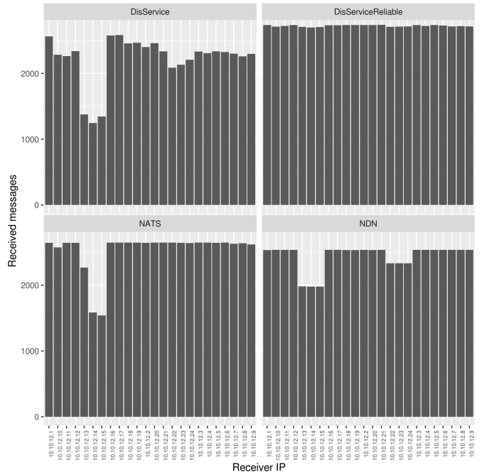
Fig. 1. Number of messages received by each node.
