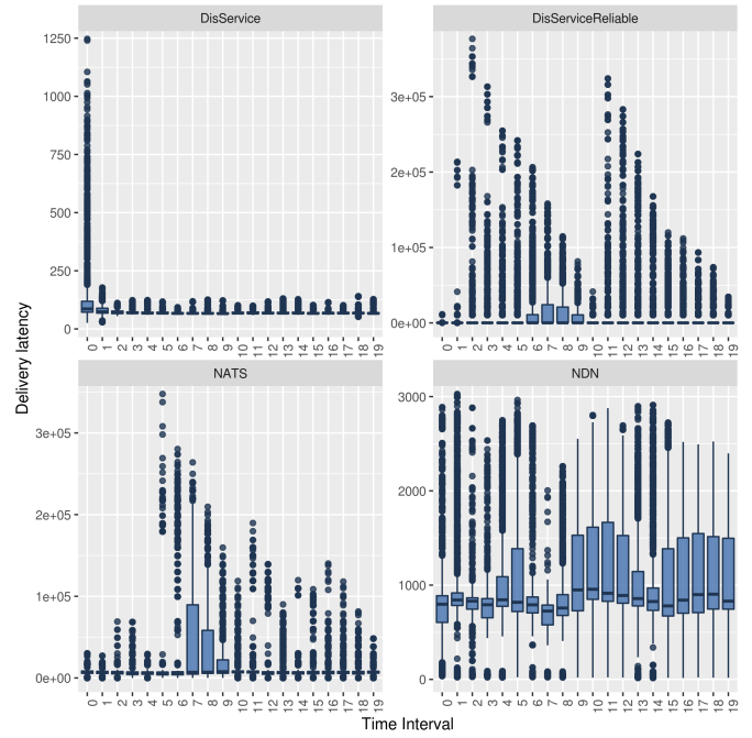
Fig. 3. Delivery latency per minute.
