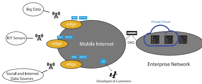
Fig. 4. MEC architecture.
