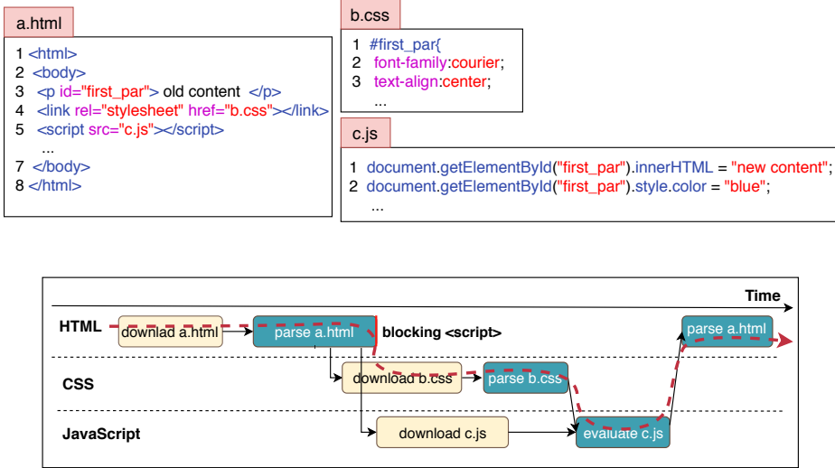
Fig. 3. (Top) An example to illustrate the dependencies between the different activities. (Bottom) Timeline showing page load activities. Black arrows represent the dependencies between activities and the red dotted line shows the page load critical path.
