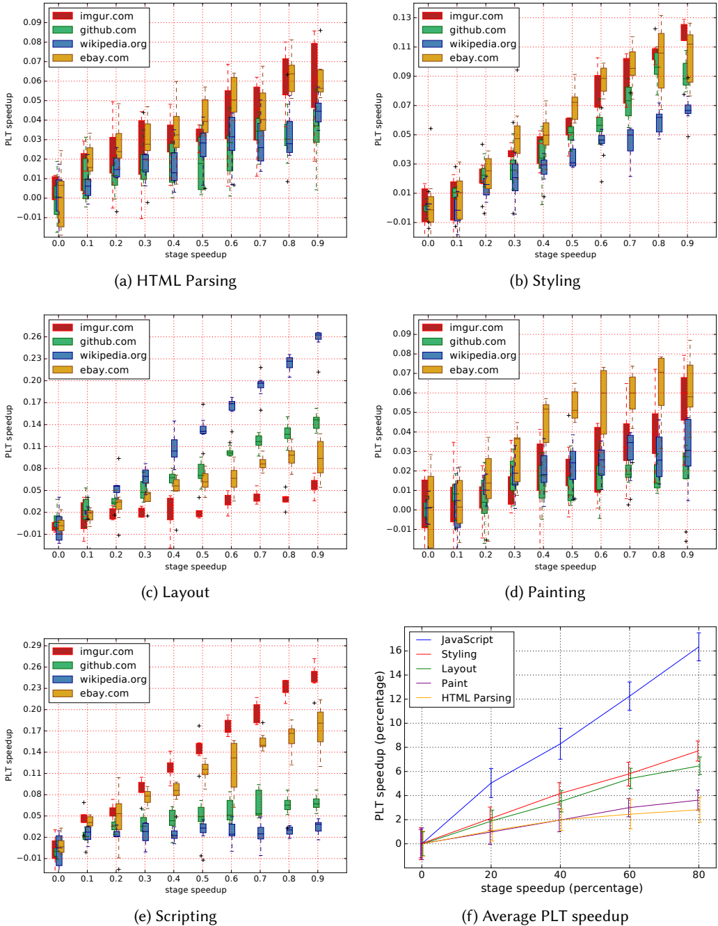
Fig. 8. (a-e) – Observed PLT improvement by accelerating browser stages namely, HTML parsing, Styling, Layout, Painting, and Scripting respectively for 4 popular example web pages. (f) – Average PLT improvement of Alexa Top 100 web pages. The boxplot displays the distribution of PLT speedup values. The boxes extend from the first to the third quartile (the 25th and 75th percentiles) with a line inside showing the median. Whiskers above and below the boxes extend from the minimum to the maximum value.
