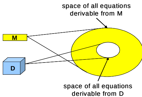
Figure 8. Relationships among 1-D models and n-D Models
