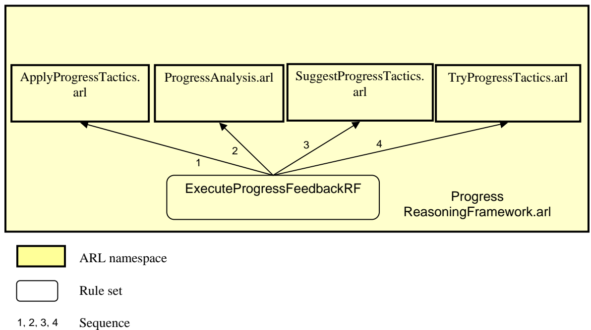
Figure 10: ARL Namespaces for Progress Feedback
