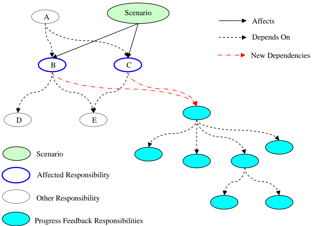
Figure 3: Responsibility Graph Linked to Scenario Before the Actions of the Reasoning Framework
