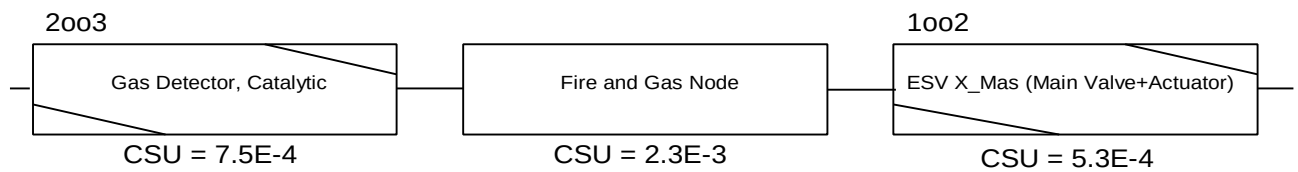
Figure 7: Reliability block diagram of the example system, small gas leakage scenario.
