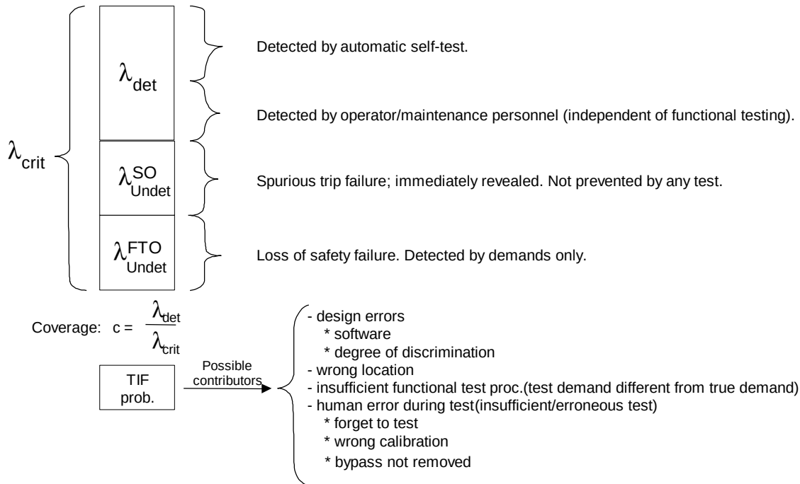
Figure 4: Interpretation of reliability parameters.
