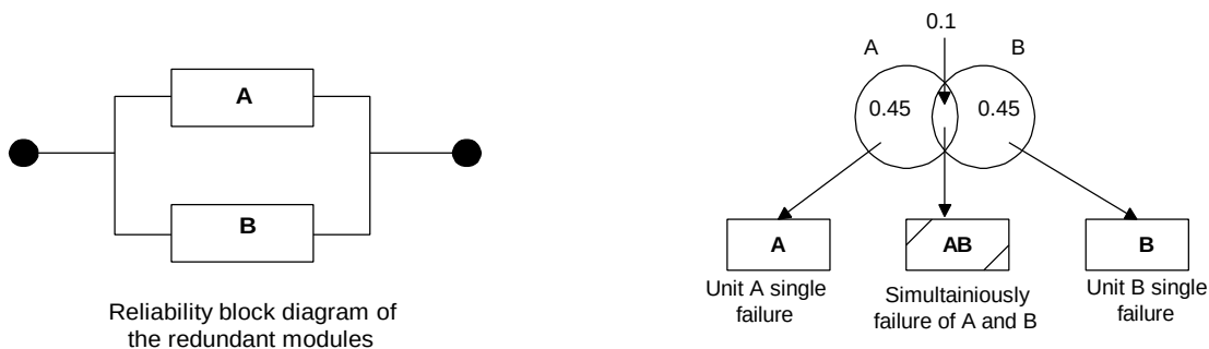
Figure 3: Example of multiplicity distribution for duplicated components.
