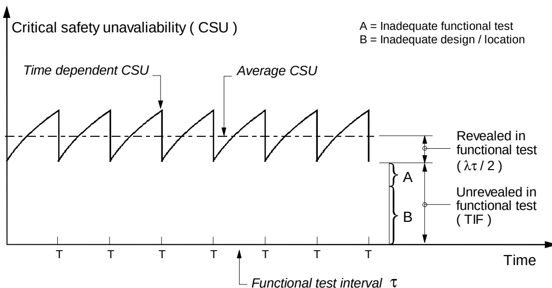
Figure 5: Contributions to the on demand failure probability, CSU.
